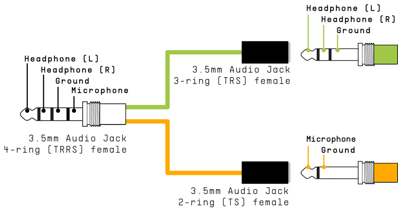
Headphone/Microphone Splitter
